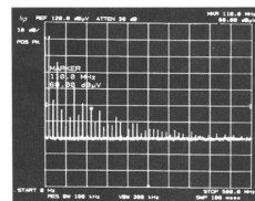
Experimentally measured spectra of 1 V, 10 MHz, 50% duty cycle
