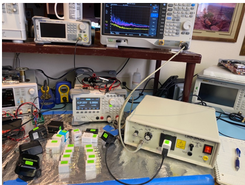
Test setup for conducted emissions.
