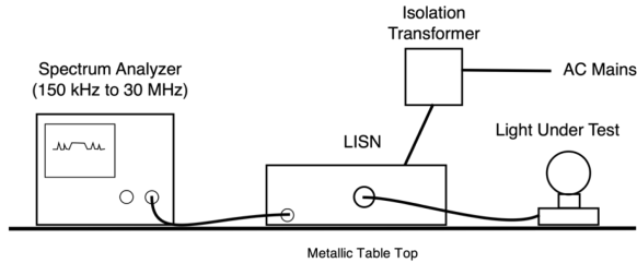
Conducted Emissions Test of LED/CFL Lamps
